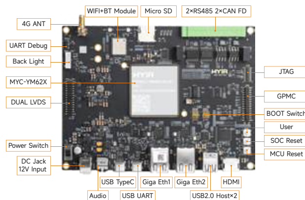
MYD-YM62X Development Board Top-view
