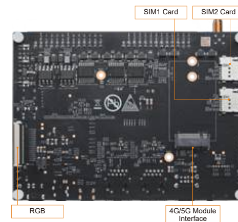
MYD-LMA35 Development Board Bottom-view
