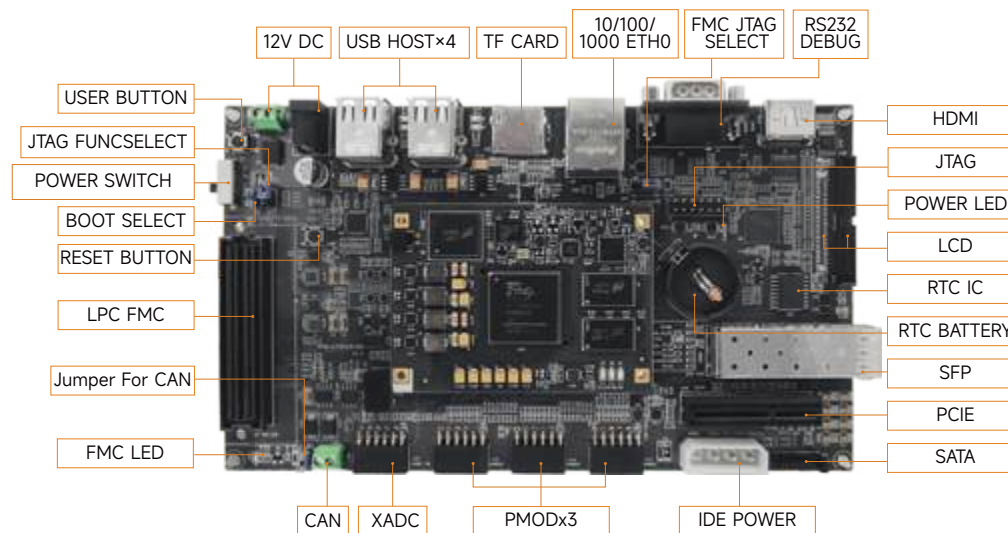
MYD-C7Z015 Development Board Top-view
