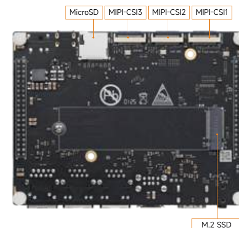
MYD-YR3562 Development Board Bottom-view
