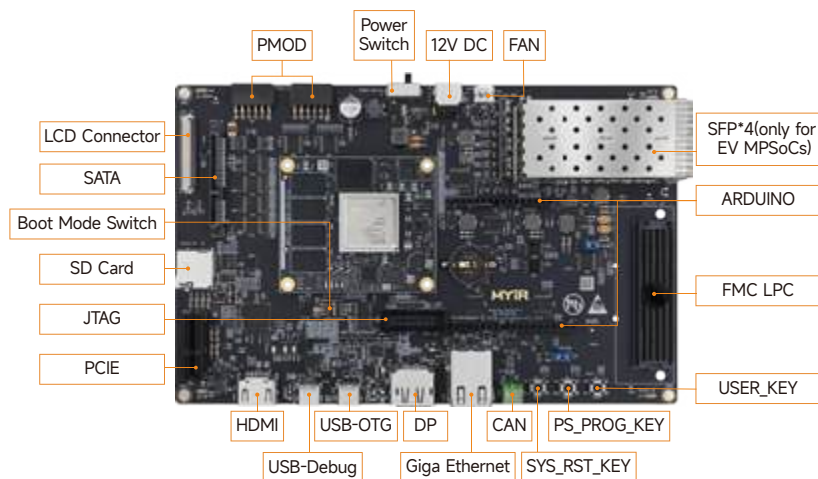
MYD-CZU3EG-V3 Development Board Top-view
