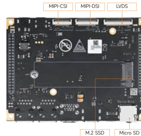
MYD-LR3568 Development Board Bottom-view
