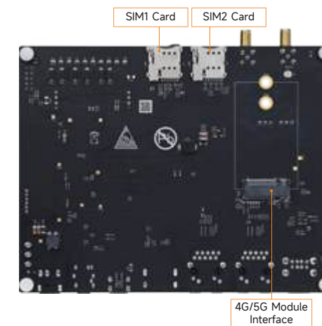
MYD-LMX91 Development Board Bottom-view
