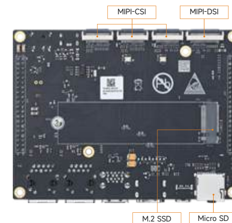
MYD-LR3576 Development Board Bottom-view
