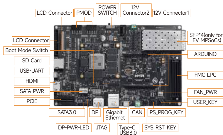
MYD-CZU3EG/4EV/5EV-V2 Development Board Top-view
