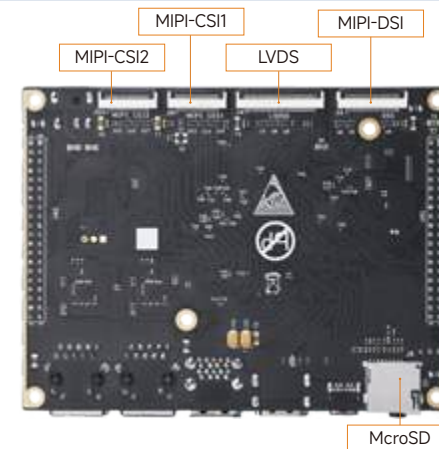
MYD-LT527 Development Board Bottom-view
