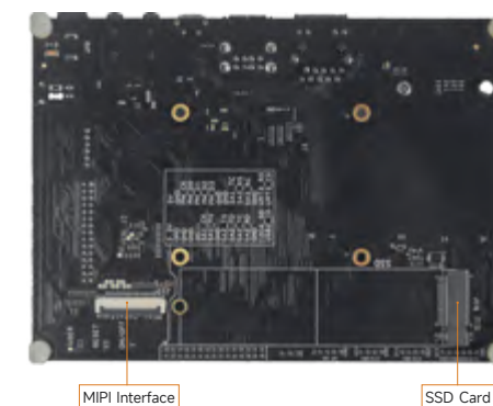
MYD-C8MMX-V2 Development Board Bottom-view
