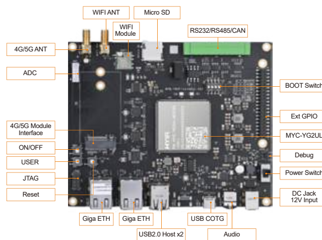
MYD-YG2UL Development Board Top-view
