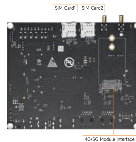
MYD-LMX9X Development Board Bottom-view
