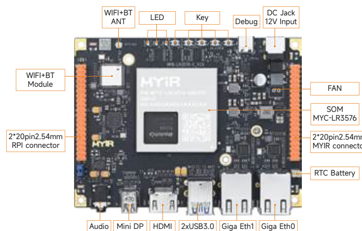
MYD-LR3576 Development Board Top-view
