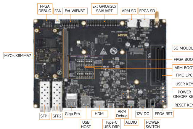
MYD-JX8MMA7 Development Board Top-view
