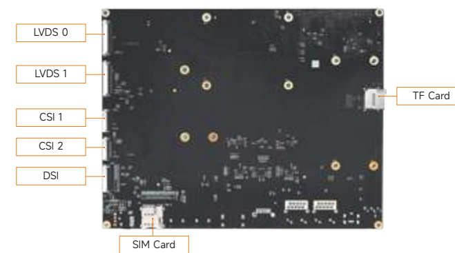
MYD-JX8MPQ Development Board Bottom-view
