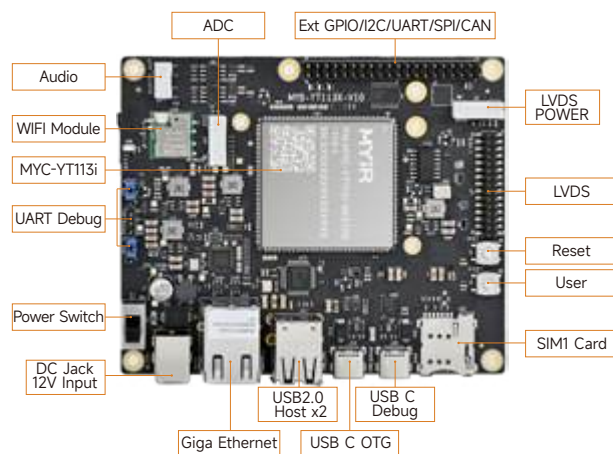
MYD-YT113i Development Board Top-view
