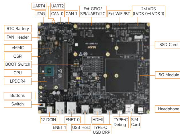
MYD-JX8MPQ Development Board Top-view
