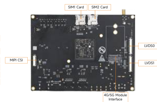
MYD-YM62X Development Board Bottom-view
