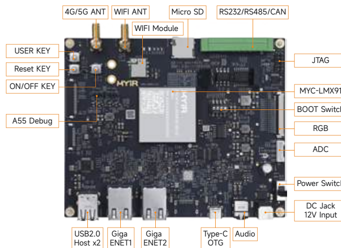
MYD-LMX91 Development Board Top-view
